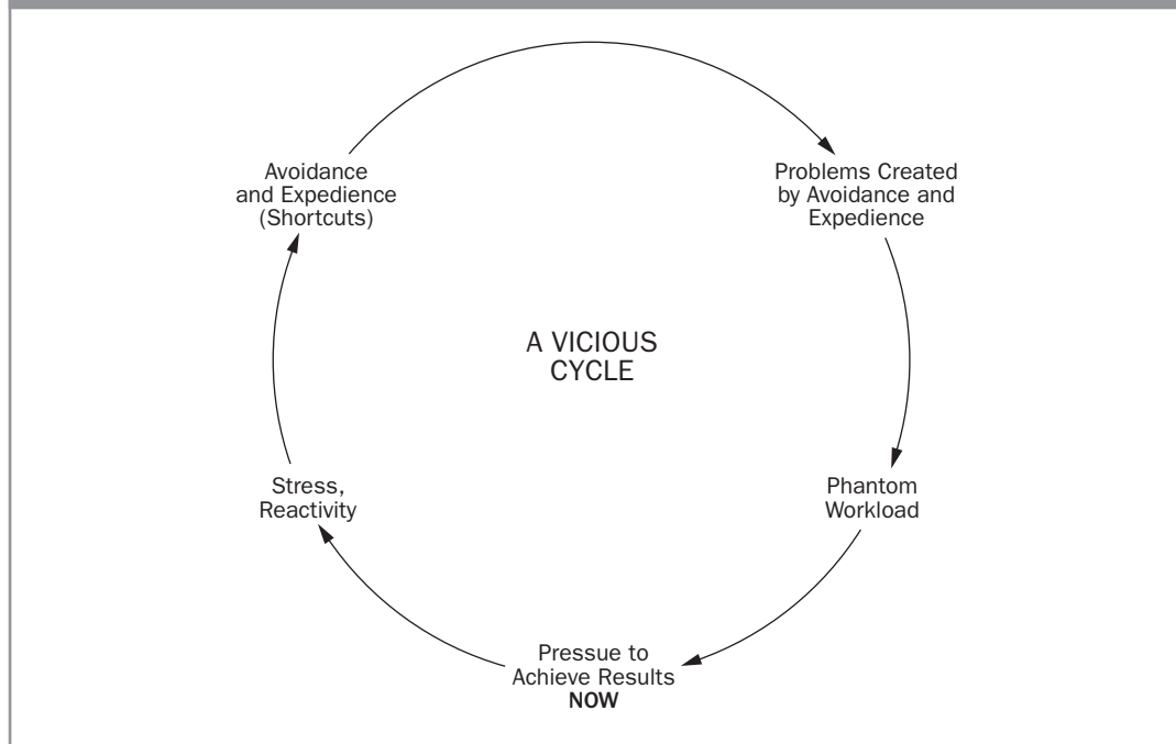
Figure 1. Phantom Workload
